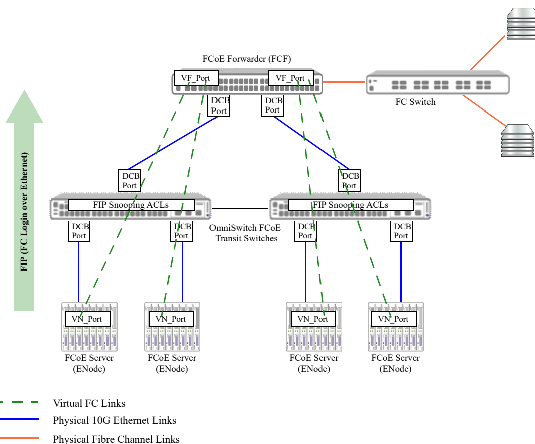
Figure 5-1 : OmniSwitch Transit Switch Connecting FCoE Endpoints
